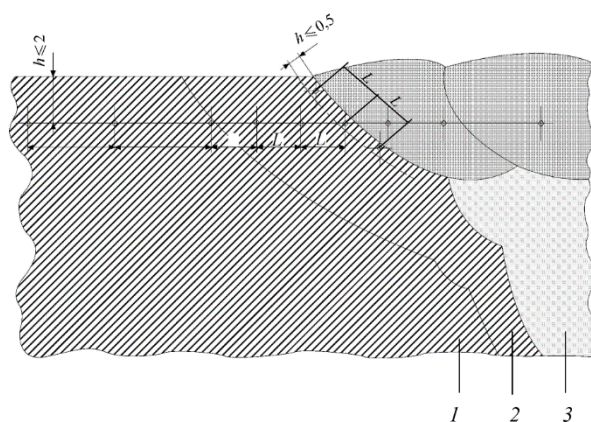
Fig. 6.4.4.5-2 Example showing the position of the indentations for hardness test in butt welds: 1 — base metal outside HAZ; 2 — HAZ; 3 — weld metal; L — distance between the centre points of the indentations: in HAZ L \geq 1,0 mm for HV10 and L \geq 0,7 mm for HV5
