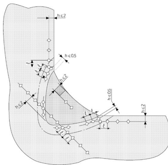
Fig. 6.4.4.5-6 Example showing the position of the indentations for hardness test in fillet welds and in T-joint welds without edge preparation
